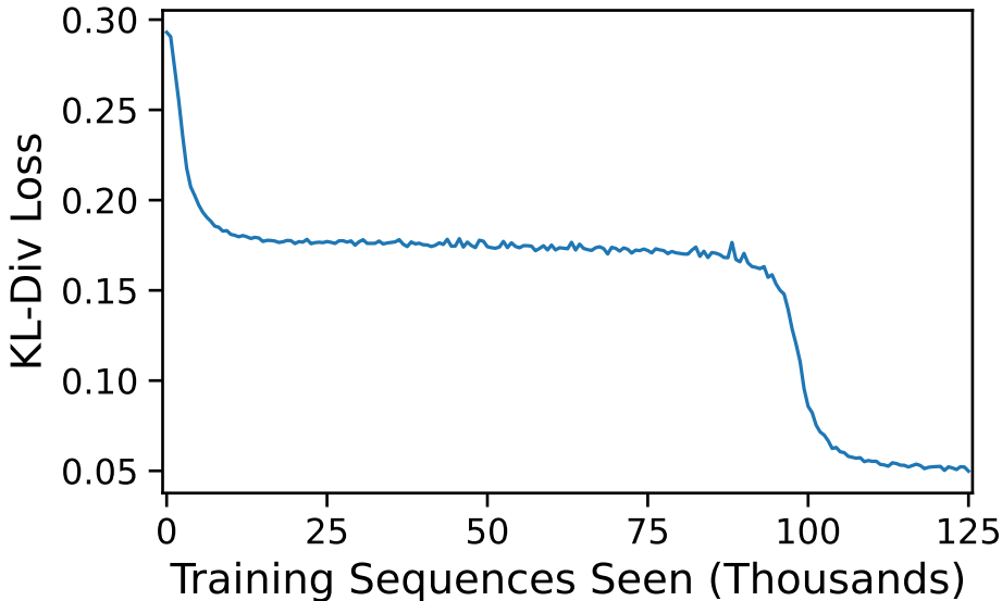
Attention-only transformer test loss on 3-state ICL-MC
